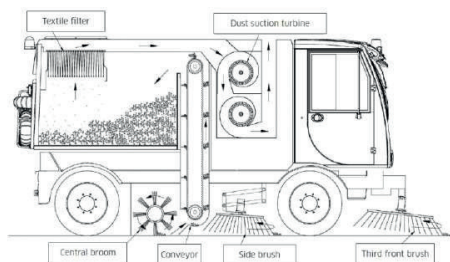
ISAL 6000 - The New Generation Sweeper
